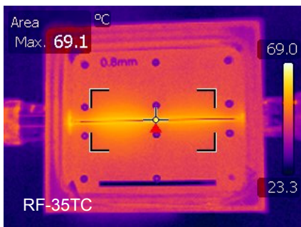
Thermal image of 0603 capacitor at the center of a microstrip (47pF/250V/C0G) assembled on RF-35TC under 200 watts applied power.
